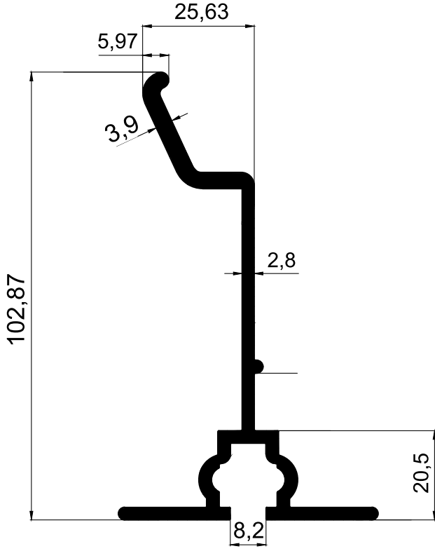
MS8021 1,634 Kg/Mt
