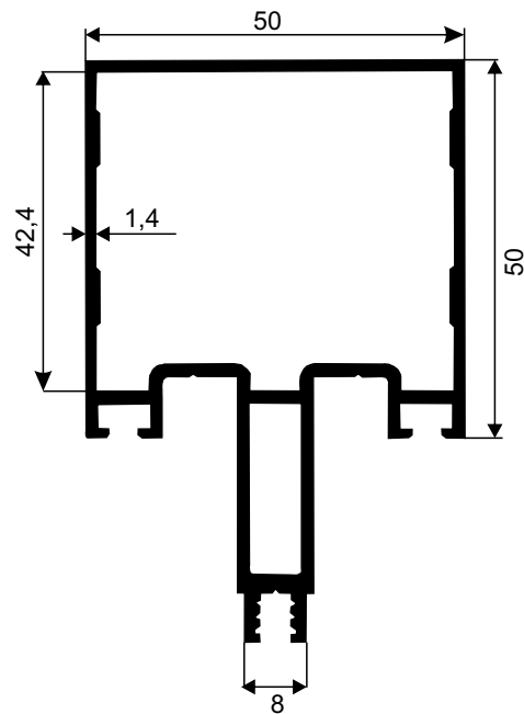
MS4014 1,222 Kg/Mt
