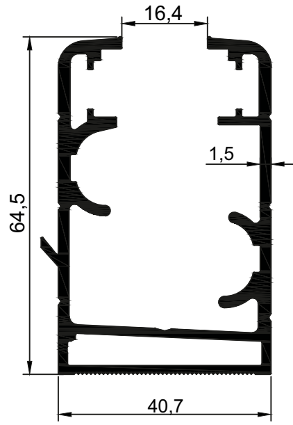
MS5002 1,430 Kg/Mt
